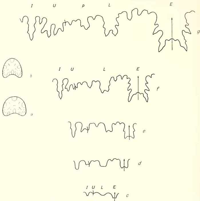
TEXT-FIG. 7. Suture development of Sc. (Otoscapites) bladenensis Schlüter, GPIT Ce 1221/14; Upper (?) Turonian, Postelberg. a , Septal surface at h = 2.5 mm, b , at h = 5 mm. c-g , Suture development, g at h = 5 mm.
